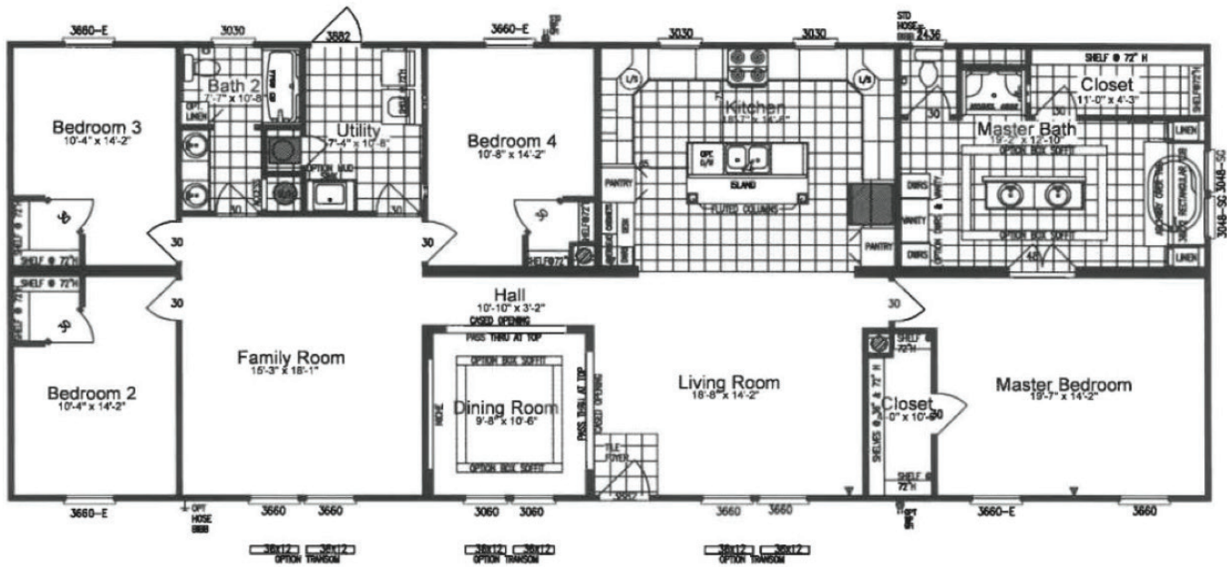
MODEL: 290TE32764B 4 BR. ~ 2 BA. 32'-0" X 80'-0" ~ 2254 SQ. FT.
